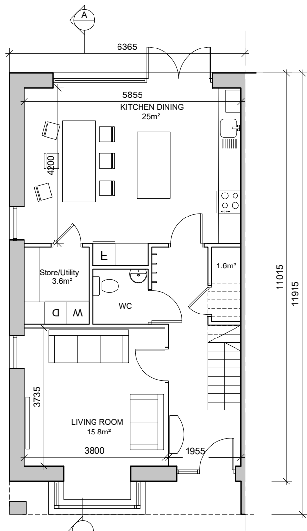
GROUND FLOOR PLAN 61 SQM 114 SQM TOTAL
