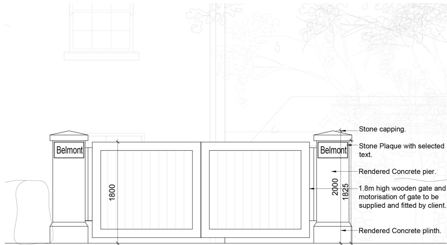
1 PROPOSED PIER & GATES ELEVATION FROM PURCHASER'S SIDE - GATES TO BELMONT SCALE 1:40
