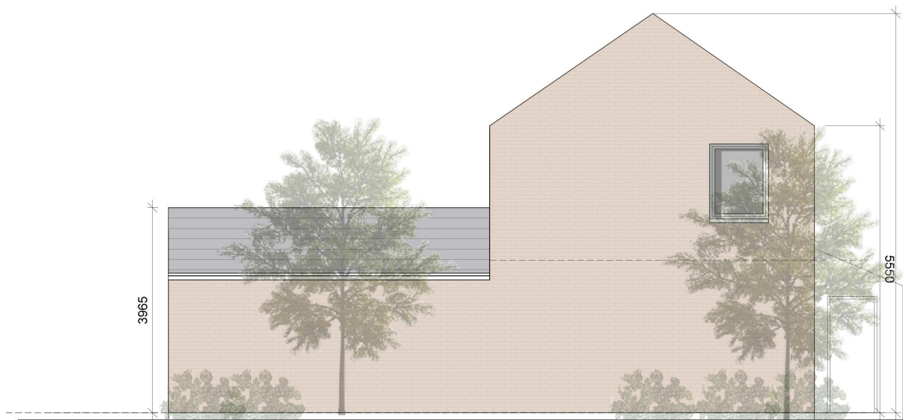
GABLE ELEVATION
