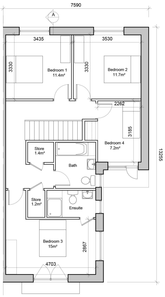
FIRST FLOOR PLAN 74 SQM
