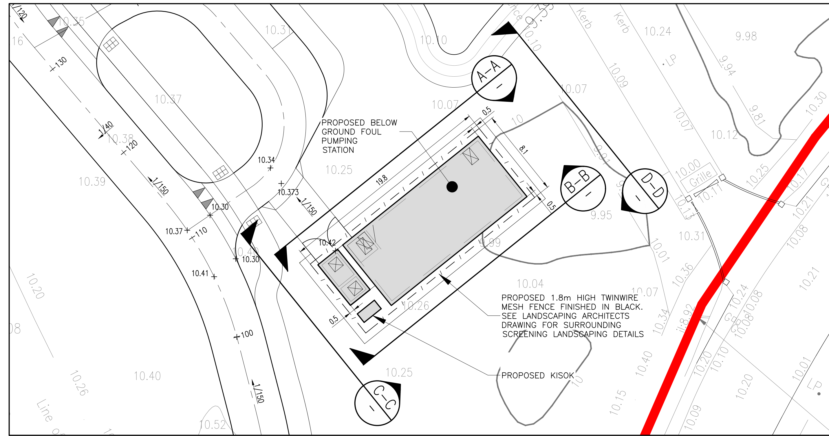
SITE PLAN – FOUL PUMPING STATION SCALE 1:200
