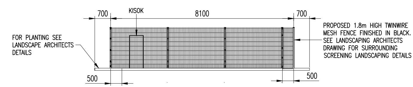
PROPOSED ELEVATION C-C SCALE 1:100
