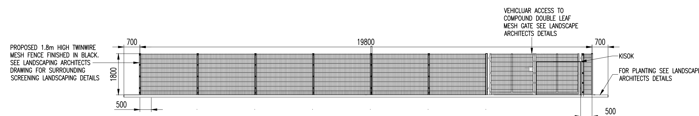
PROPOSED ELEVATION A-A SCALE 1:100
