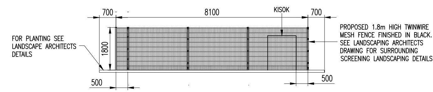
PROPOSED ELEVATION D-D SCALE 1:100
